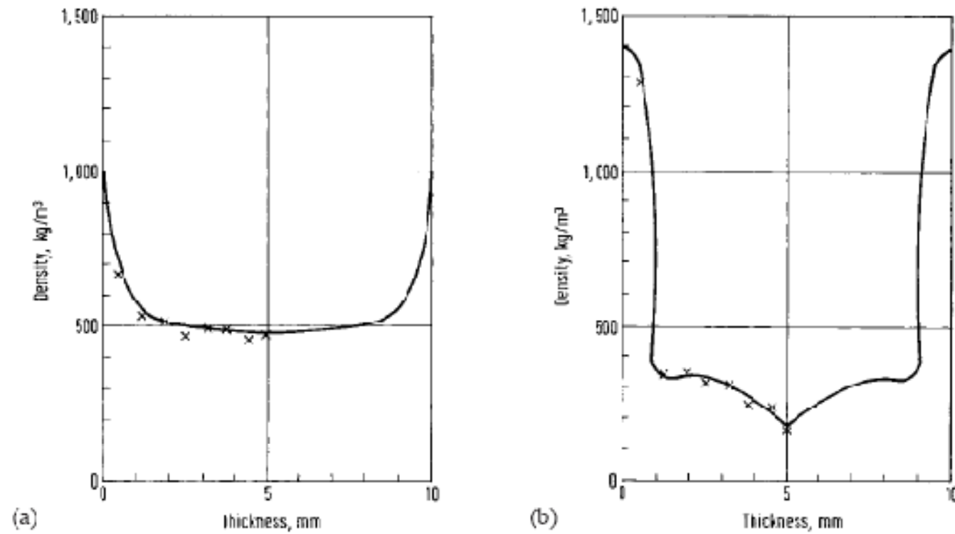
Figure 9.12 Comparison of foam density distribution. (a) Free foam; (b) Celuka process
