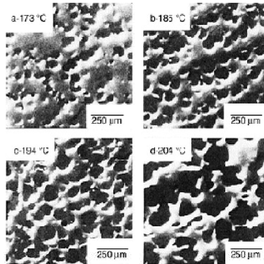
Figure 9.14 Influence of melt temperature on the cell structure of a PVC foam [53] (Courtesy of Society of Plastics Engineers)
